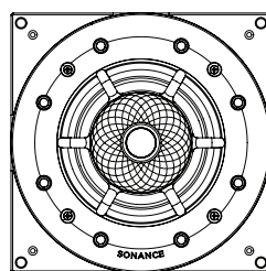
Front View Square Adaptor
