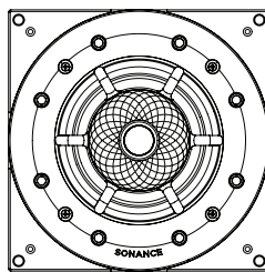
Front View Square Adaptor
